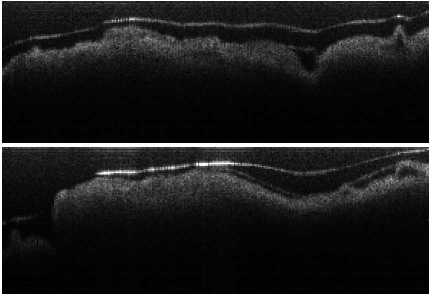
Figure 2. Typical B-scans (mid-IR OCT) of an oil painting sample
