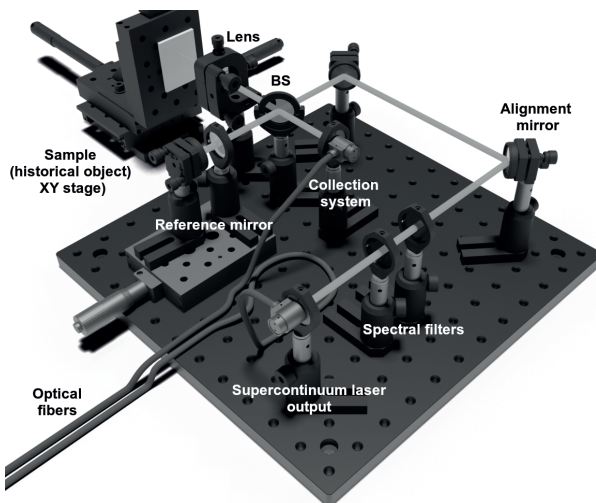
Figure 1. Optical arrangement of the system
